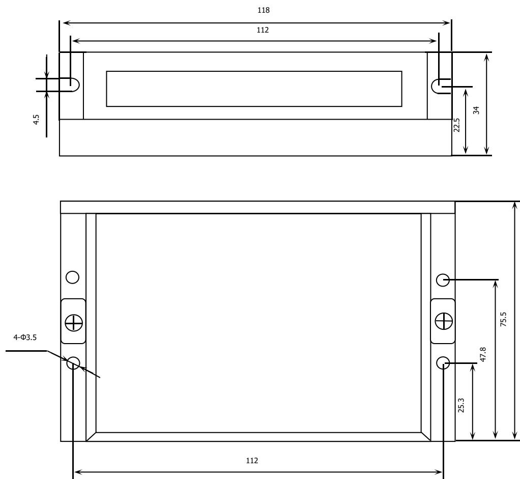
Drawing 1 Installation dimension diagram (Unit:mm)
